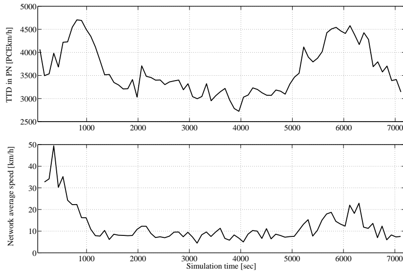
Figure 6: Case study 1: network performances
