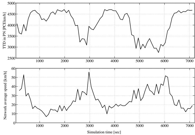
Figure 9: Case study 2: network performances
