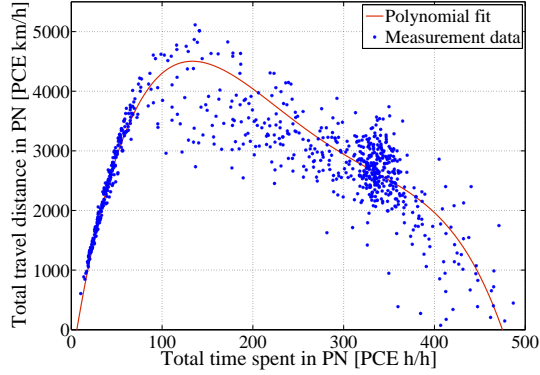
Figure 2: Fundamental diagram of the protected network
