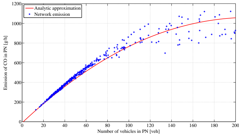
Figure 13: Network emission as a function of number of vehicles
