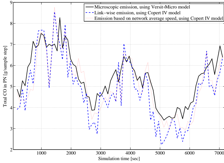
Figure 10: Case study 2: network emissions
