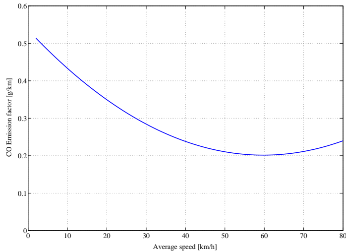
Figure 11: Emission factor function of CO pollution (passenger car equipped with an Euro 5 gasoline engine, under 1.4 l)
