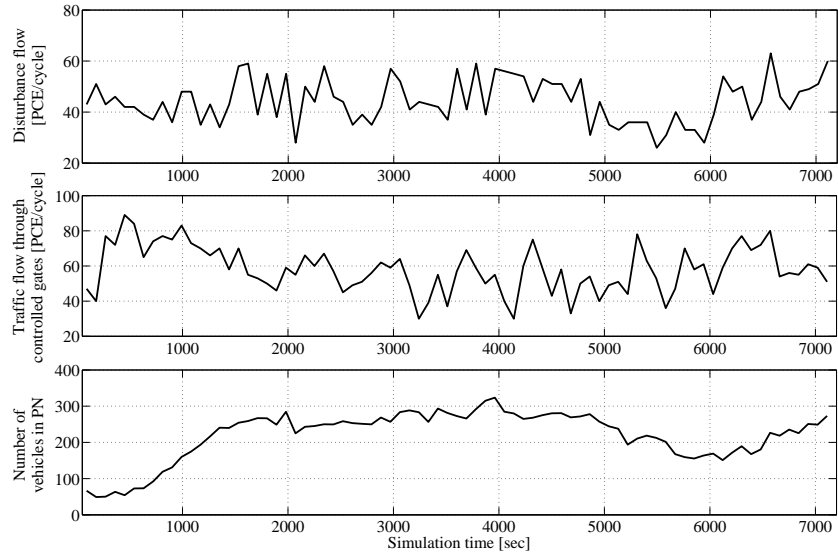
Figure 5: Case study 1: gate inputs and number of vehicles in PN
