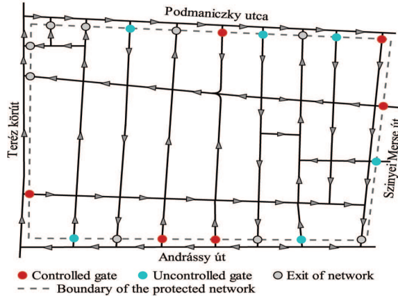
Figure 1: Network layout
