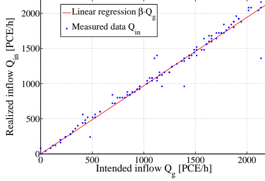
Figure 4: Linear regression for parameter \beta
