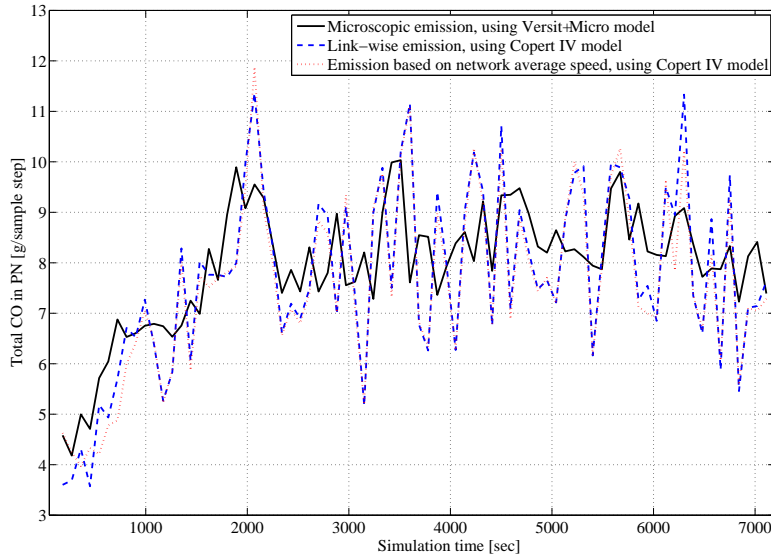
Figure 7: Case study 1: network emissions
