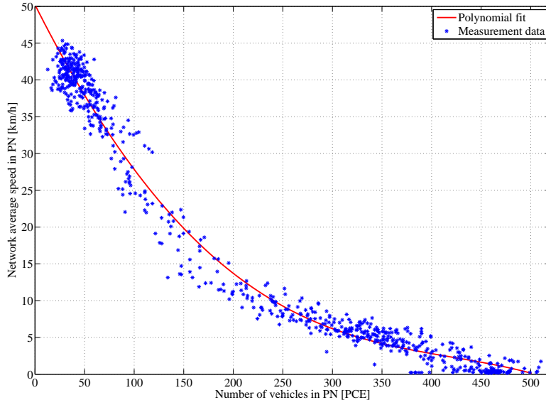
Figure 12: Network average speed function
