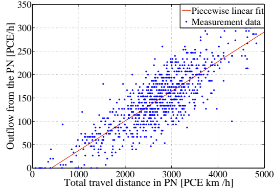
Figure 3: Linear regression for parameter \Gamma
