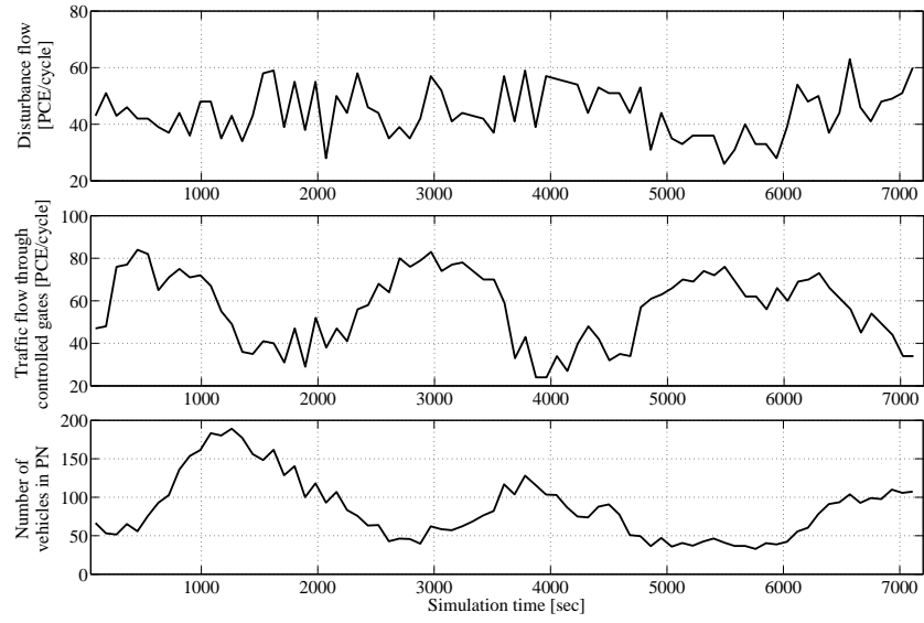
Figure 8: Case study 2: gate inputs and number of vehicles in PN
